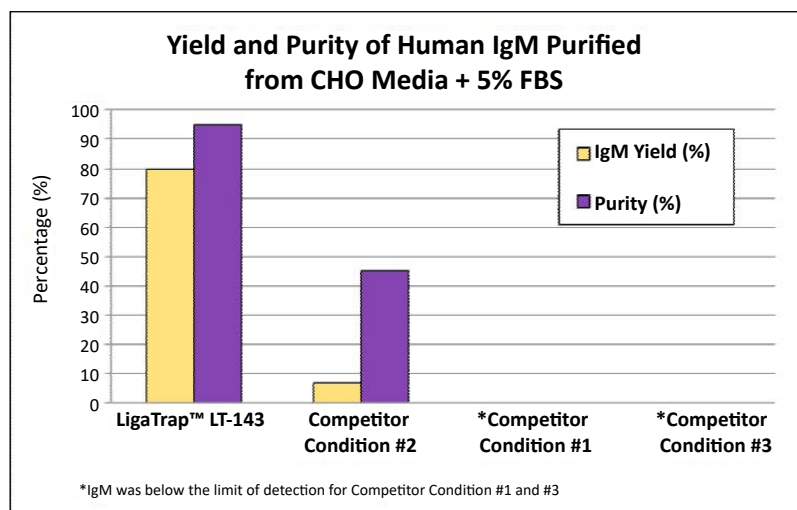
Figure 1. Percent yield of purified IgM was calculated from a load of 10mg Hu IgM per ml of resin. Percent purity was assessed by HPLC analysis.
