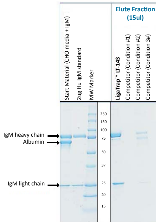
Figure 2. 15ul of each elute fraction was assayed by reducing SDS-PAGE and stained with Coomassie dye.
